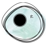
Cellule normale
